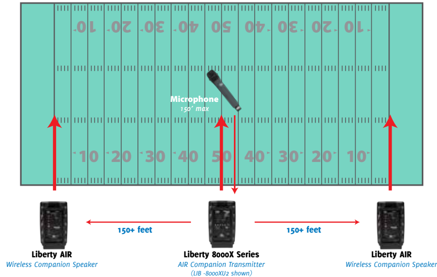
Anchor AIR System Arrangement
